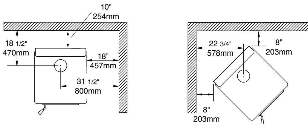
Figure 17: Summit LE Minimum clearances - Mobile Home.
