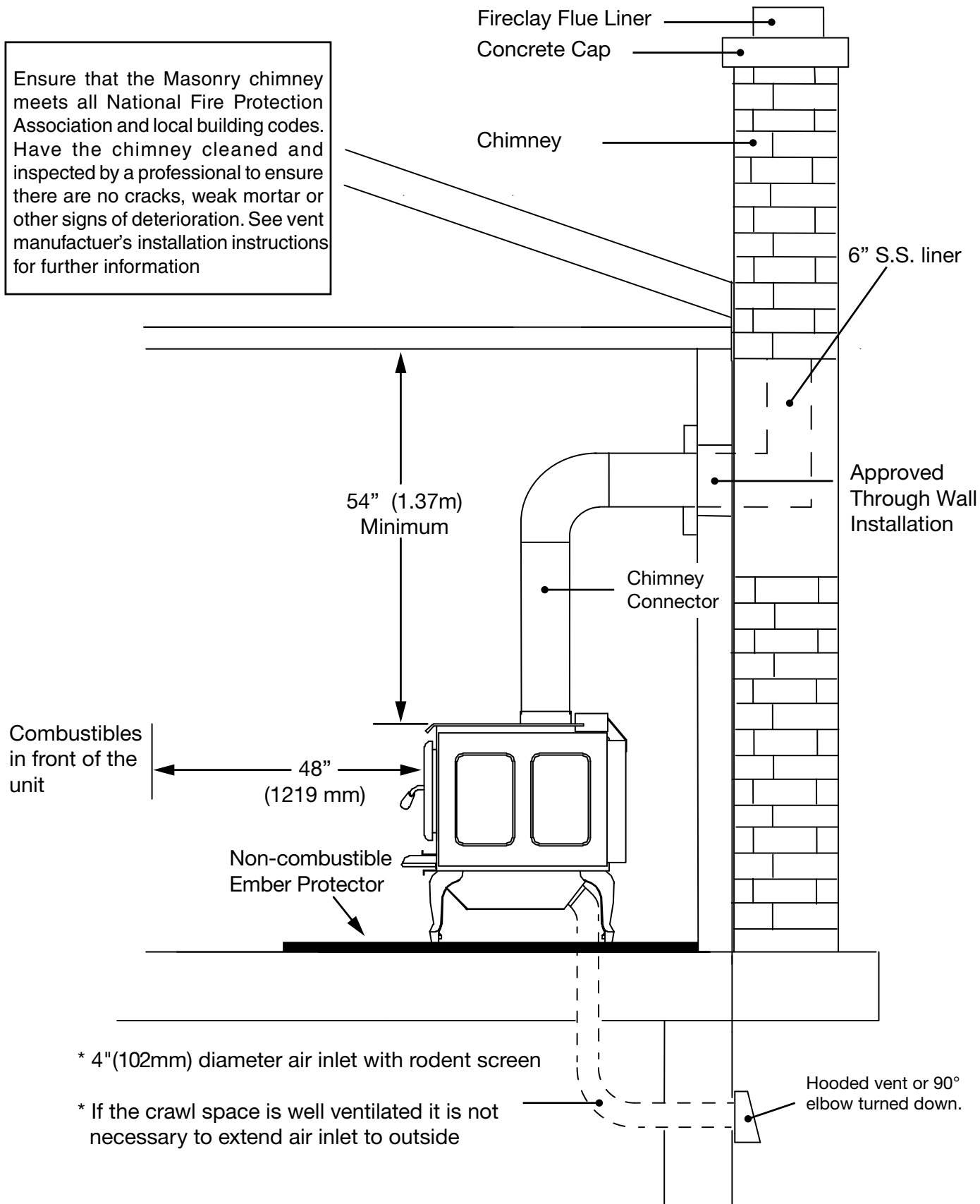
Figure 12: Summit LE Venting to a masonry chimney.
