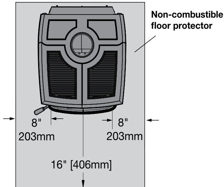
Figure 2: T5 Floor protector - USA
