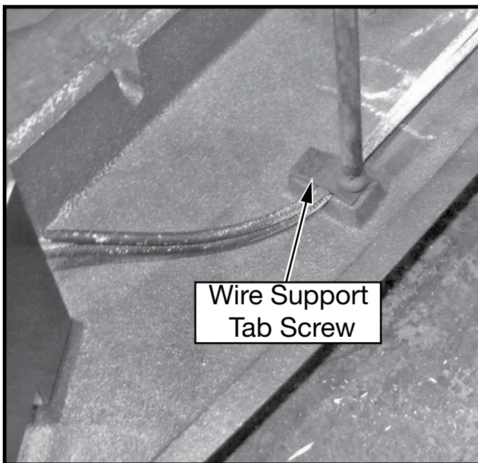
Figure 23: Wire Guides.
