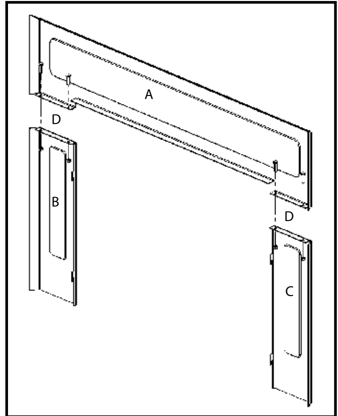
Figure 12: Surround assy.
