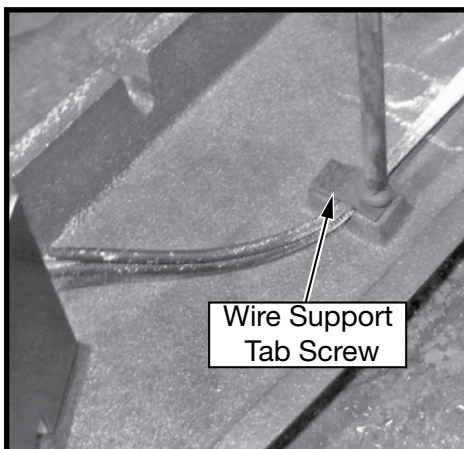
Figure 16: Wire Guides.
