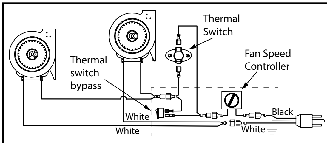
Figure 8: Wiring Diagram - Insert LE.
